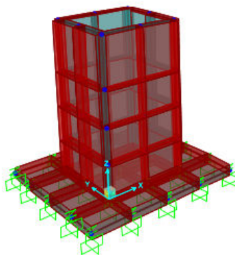
FIG 3 - Structure 3D Model in SAP2000(Oily Sump Pit)
