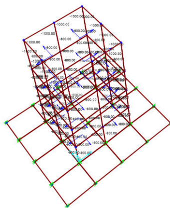
FIG 20 - Applied hydrostatic pressure on walls(Oily Sump Pit)
