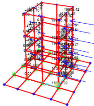
FIG 26 - Applied hydrodynamic force on wall(Oily sump pit)
