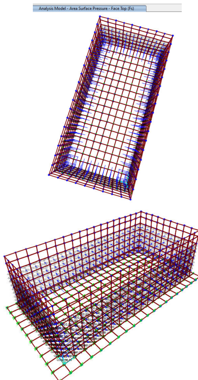
FIG 19 - Applied hydrostatic pressure on walls(SU-2201B)
