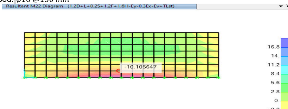
FIG 30 - Resultant M22 Diagram(ton-m)
