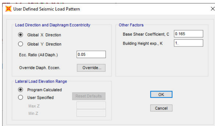
FIG 7 - X Direction Seismic Load
