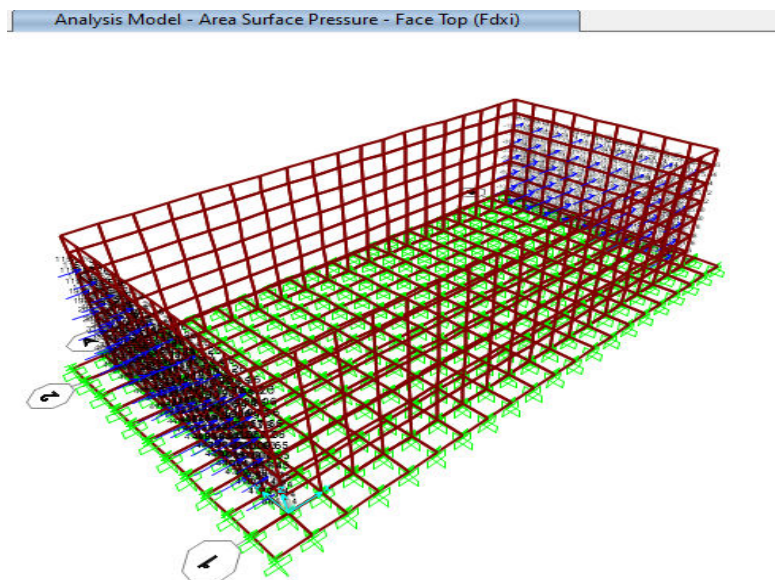
FIG 21 - Applied hydrodynamic force on wall(Fdxi)
