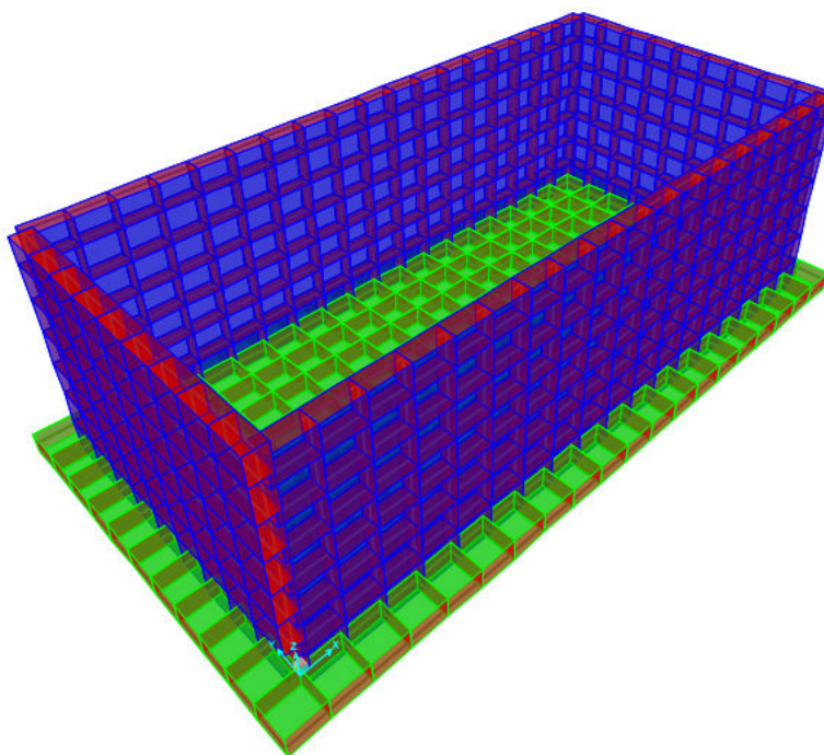
FIG 2 - Structure 3D Model in SAP2000(SU-2201B)
