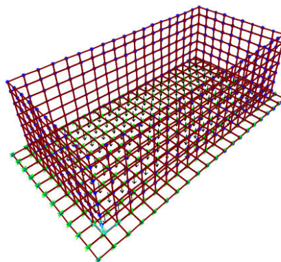
FIG 27 - applied oil weight on bottom of sump(2530kg/m2)
