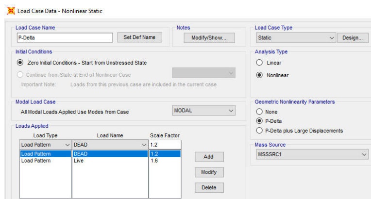
FIG 29 - P-Delta
