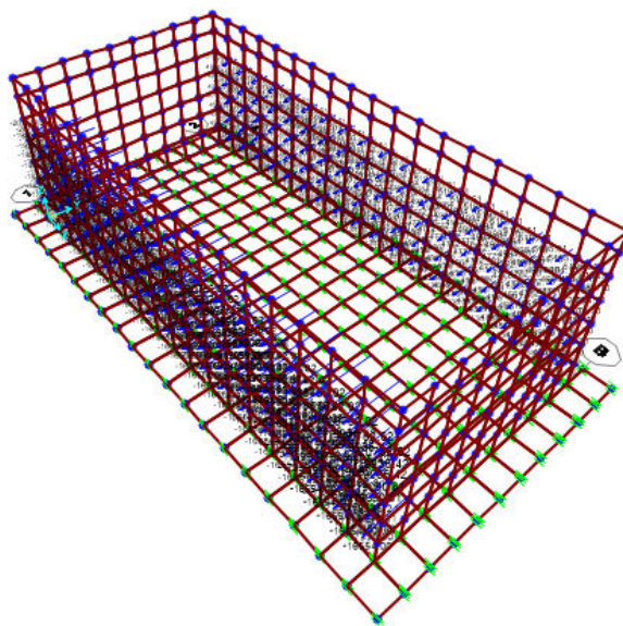
FIG 23 - Applied hydrodynamic force on wall(Fdyc)
