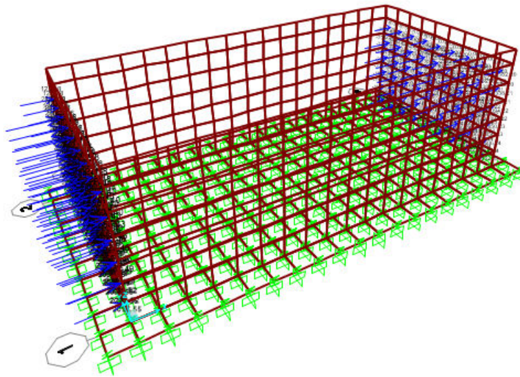
FIG 24 - Applied hydrodynamic force on wall(Fdx)
