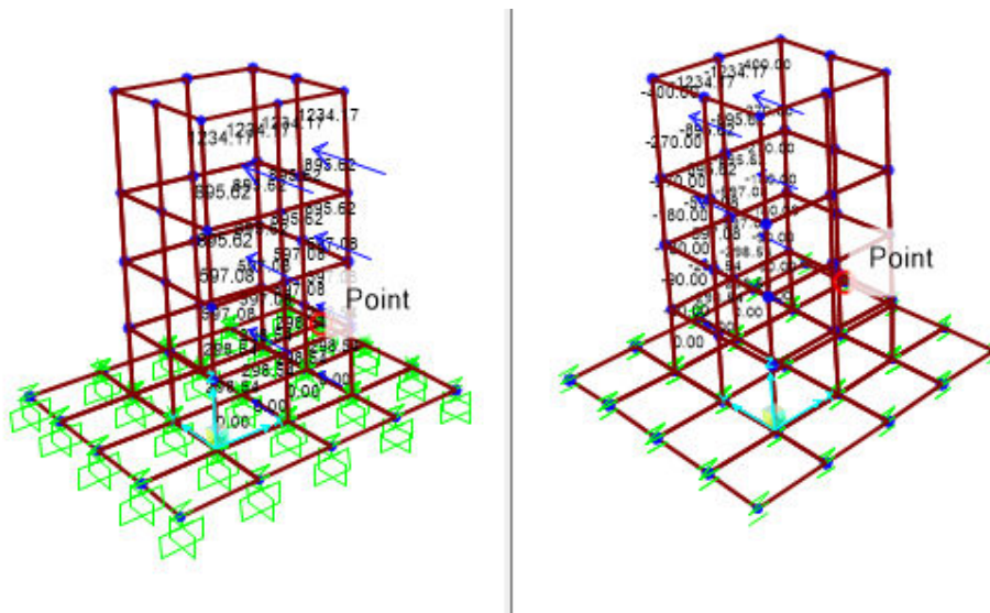
FIG 17 - Applied Lateral Dynamic Pressure of soil on Oily Sump Pit (X direction)
