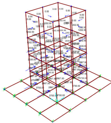
FIG 14 - Applied Lateral Soil Pressure(Oily Sump Pit)
