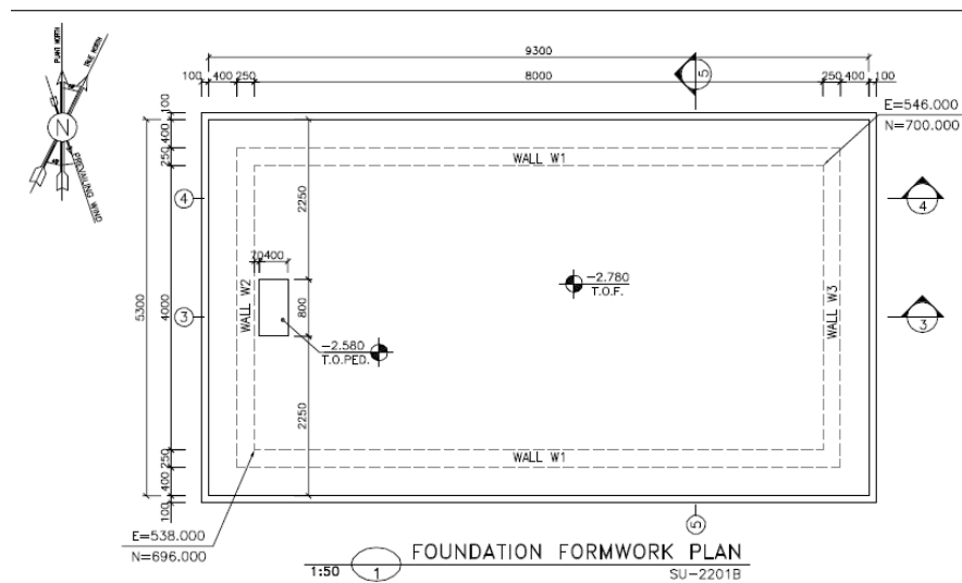
FIG 4 - Foundation Formwork Plan(SU-2201B)
