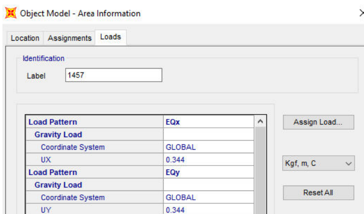
FIG 12 - Applied wall seismic coefficient
