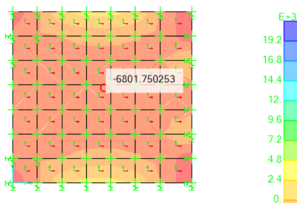
Figure 13-M22 Diagram on bottom of Pit
