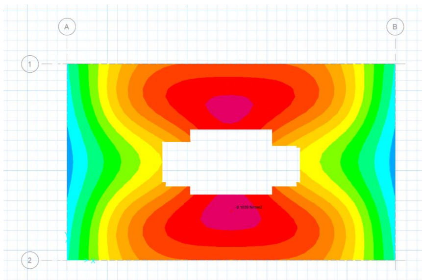
Figure 4 –Soil Pressure under service Load Combination(0.118 N/mm 2 )
