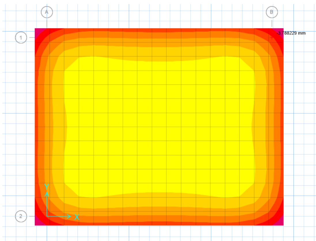
Figure18 –Displacement under service load combination(3.78 mm)
