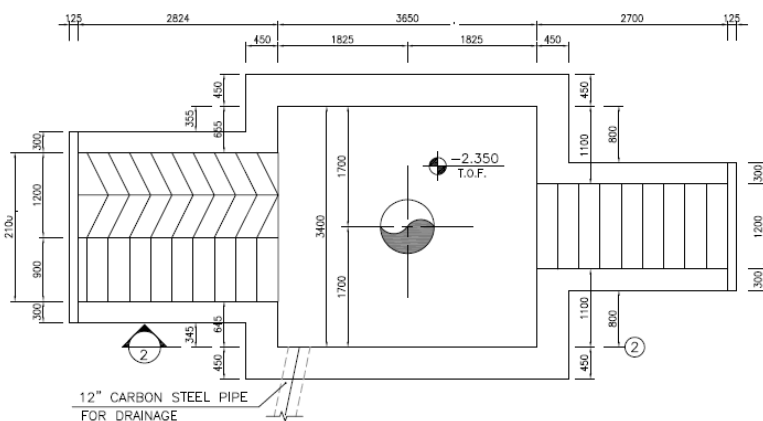
Figure 1-Cellar pit Area
