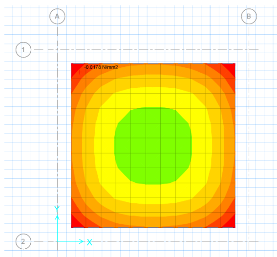
Figure25–soil Pressure under service load combination(max=0.0178 N/mm2)
