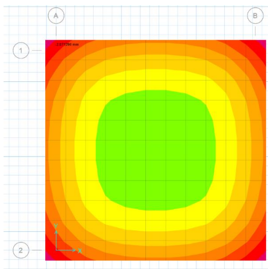
Figure24 –Displacement under service load combination(1.31 mm)
