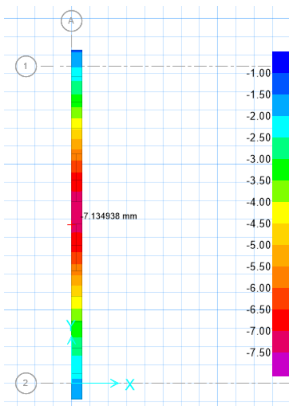
Figure38 –soil displacement under service load combination(7.13mm)
