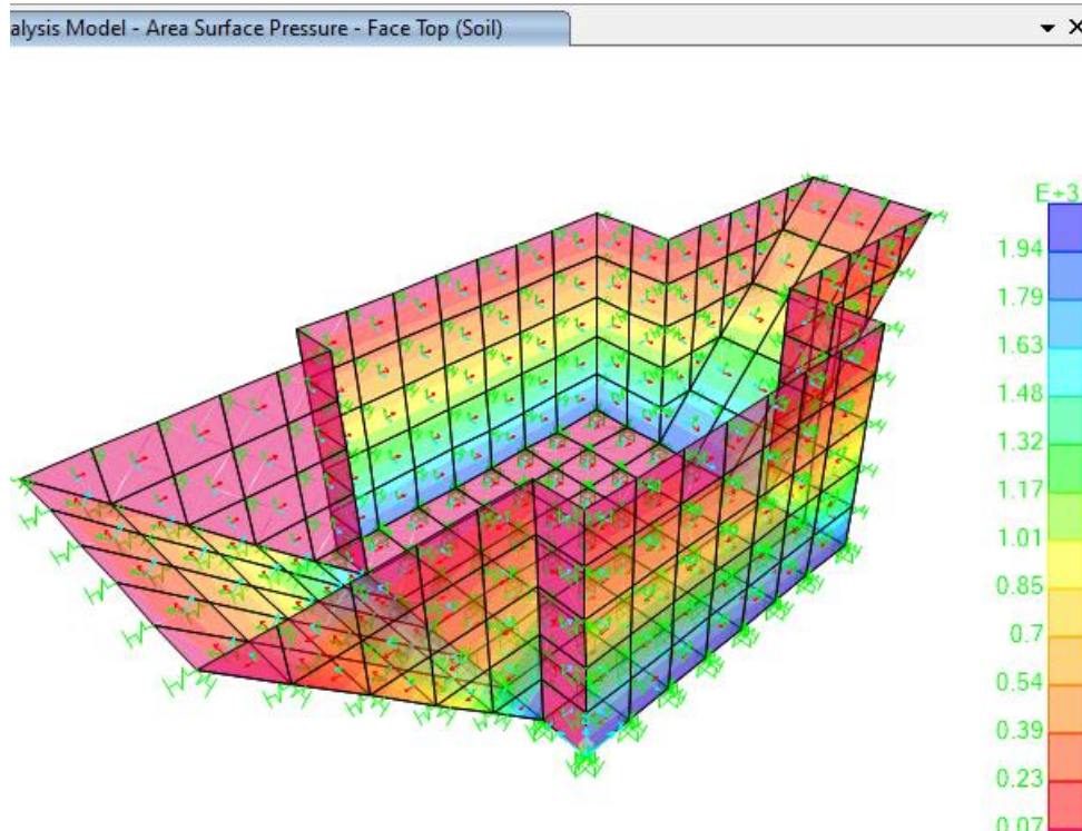
Figure 8 –Applied Soil Pressure Load
