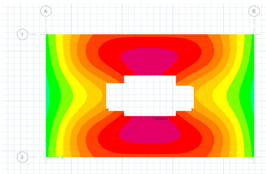
Figure 3 –Settlement Of foundation under service Load Combination(mm)
