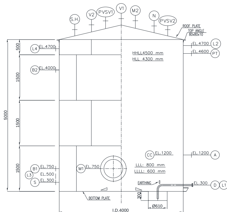
ELEVATION VIEW
