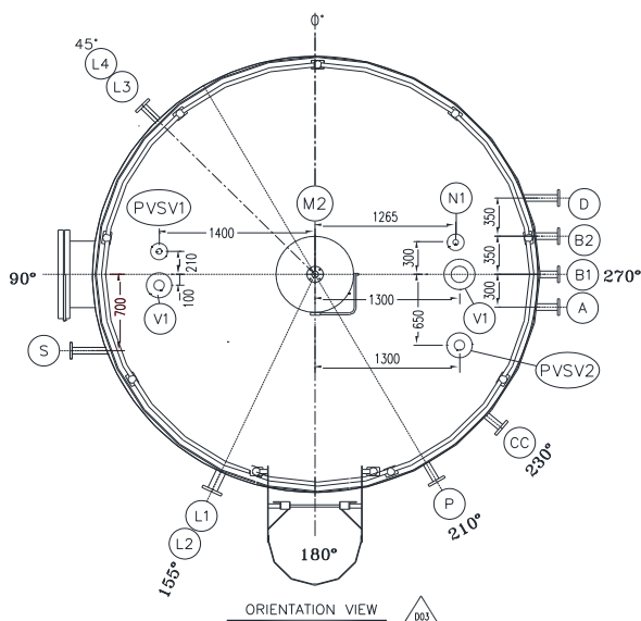
ORIENTATION VIEW
