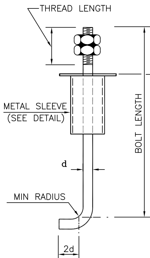
TYPE "LS"
