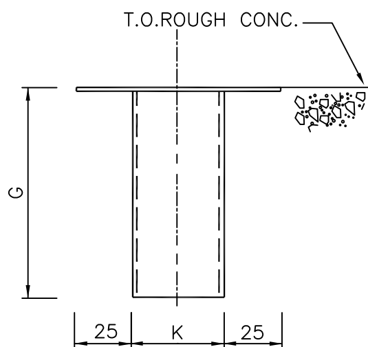
ELEVATION OF SLEEVE
