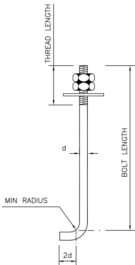
TYPE "L"
