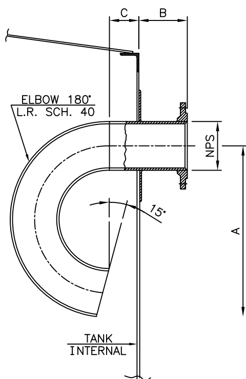
TYPE "A"
