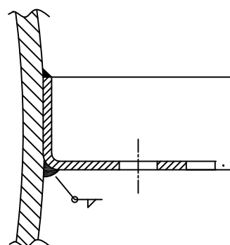
SEC. "A-A"
