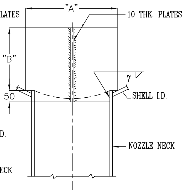
TYPE-B
