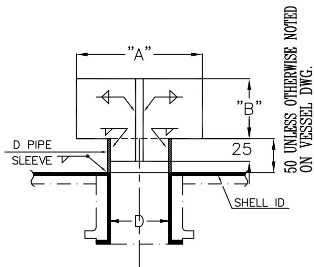
TYPE-C FOR LINED VESSELS
