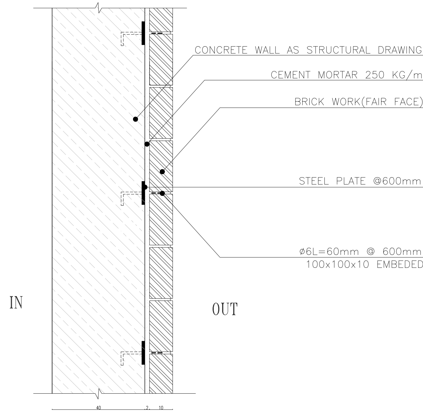
DETAIL 06 (CONNECTING BRICK FACE TO CONCRETE WALL) Sc:1/10
