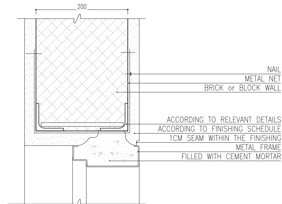
DETAIL 09 Sc:1/5
