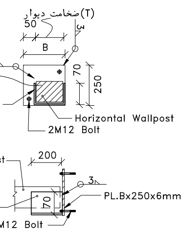
DETAIL-4
