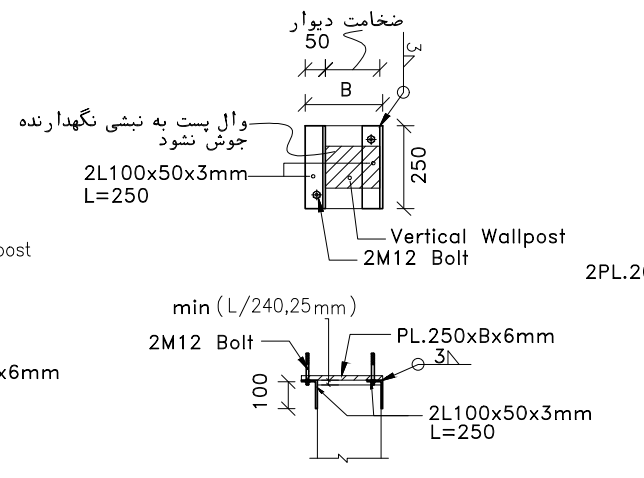
DETAIL-2
