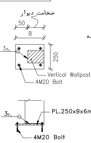
DETAIL-1b
