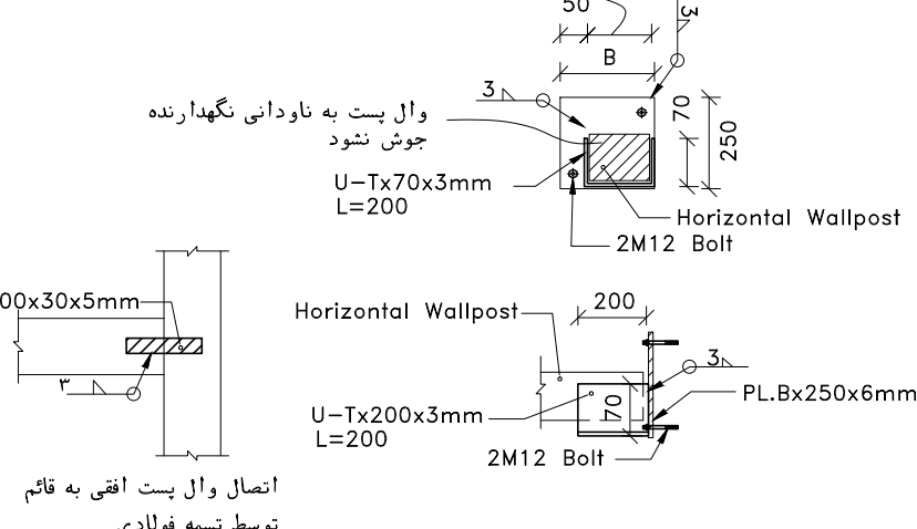
DETAIL-4
