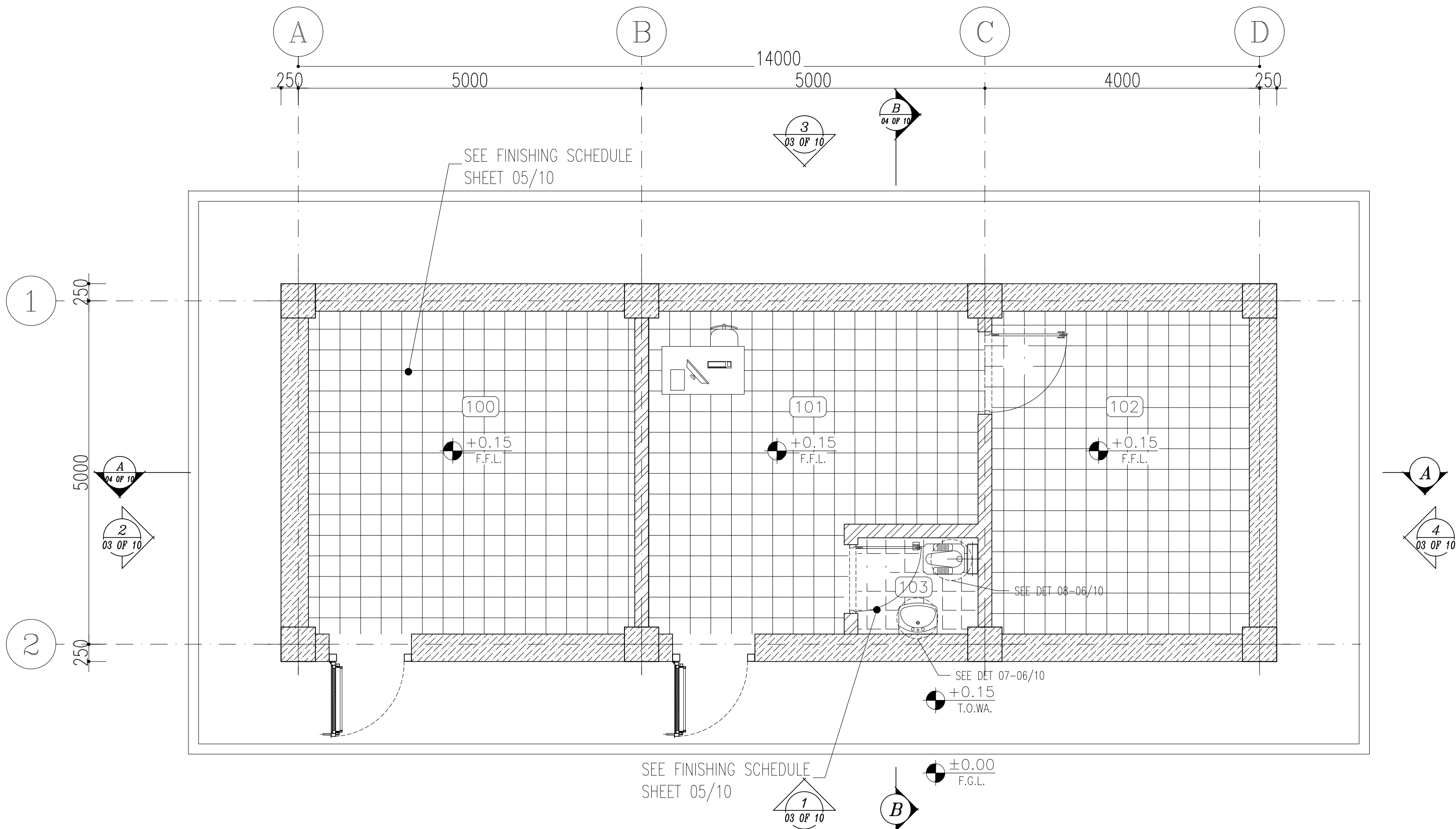
2 FLOORING PLAN SC.1:50
