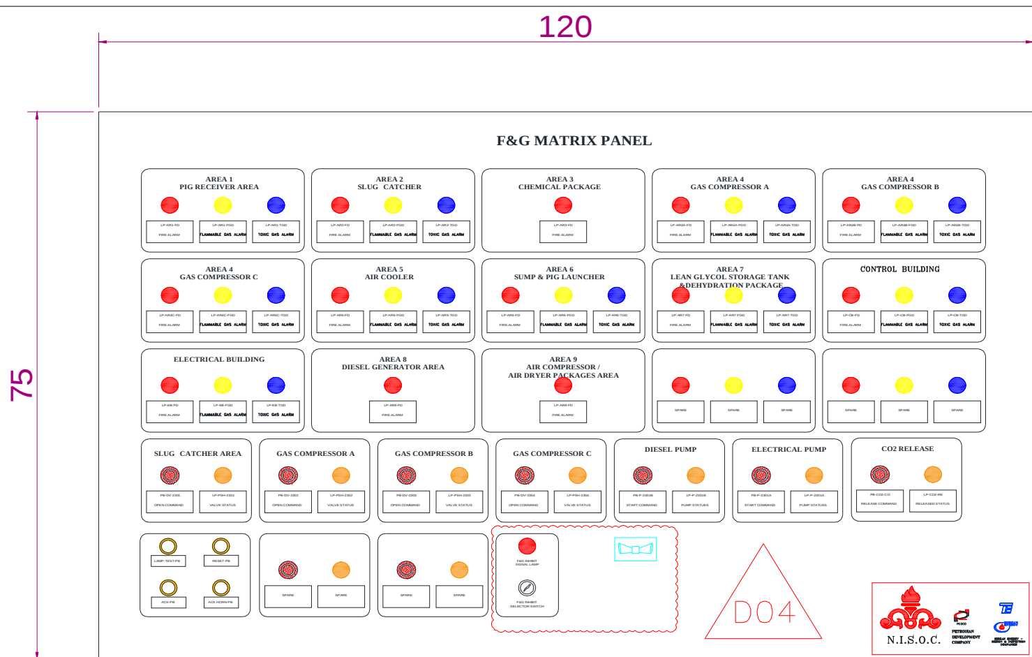
SCHEMATIC OF F&G MATRIX PANEL ESTIMATED DIMENSION 120cmX75cm (TO BE FINALIZED BY VENDOR)
