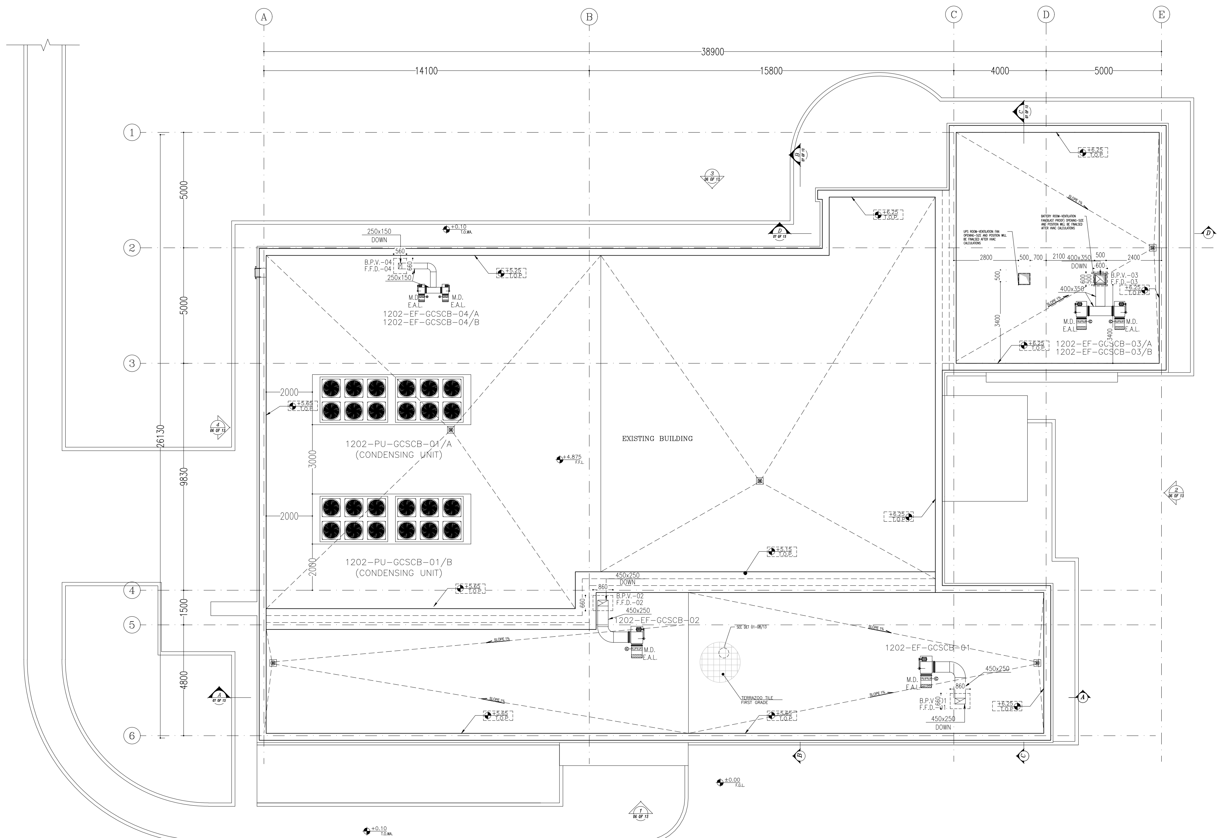
SC.1:100 5 ROOF PLAN
