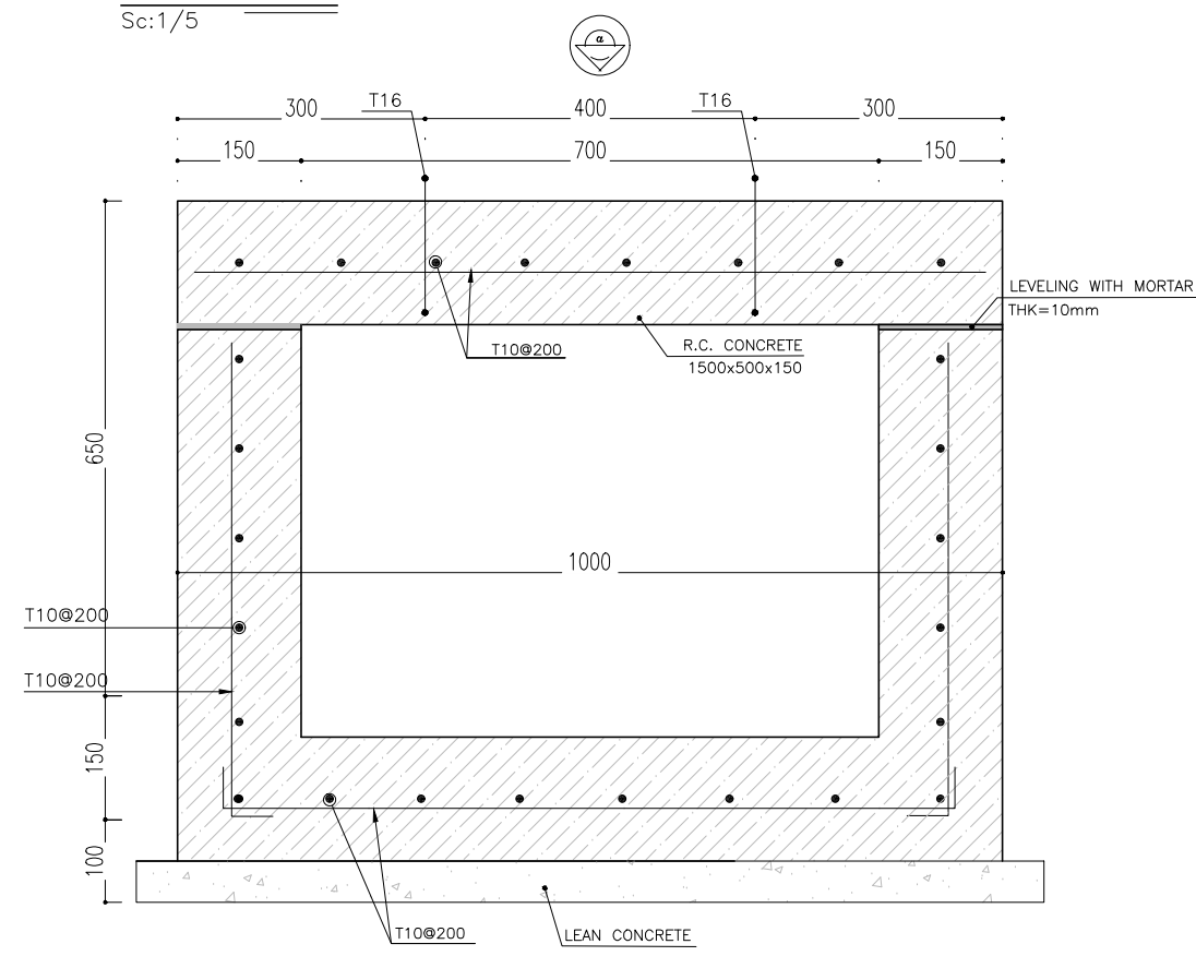
DETAIL 11 Sc:1/10
