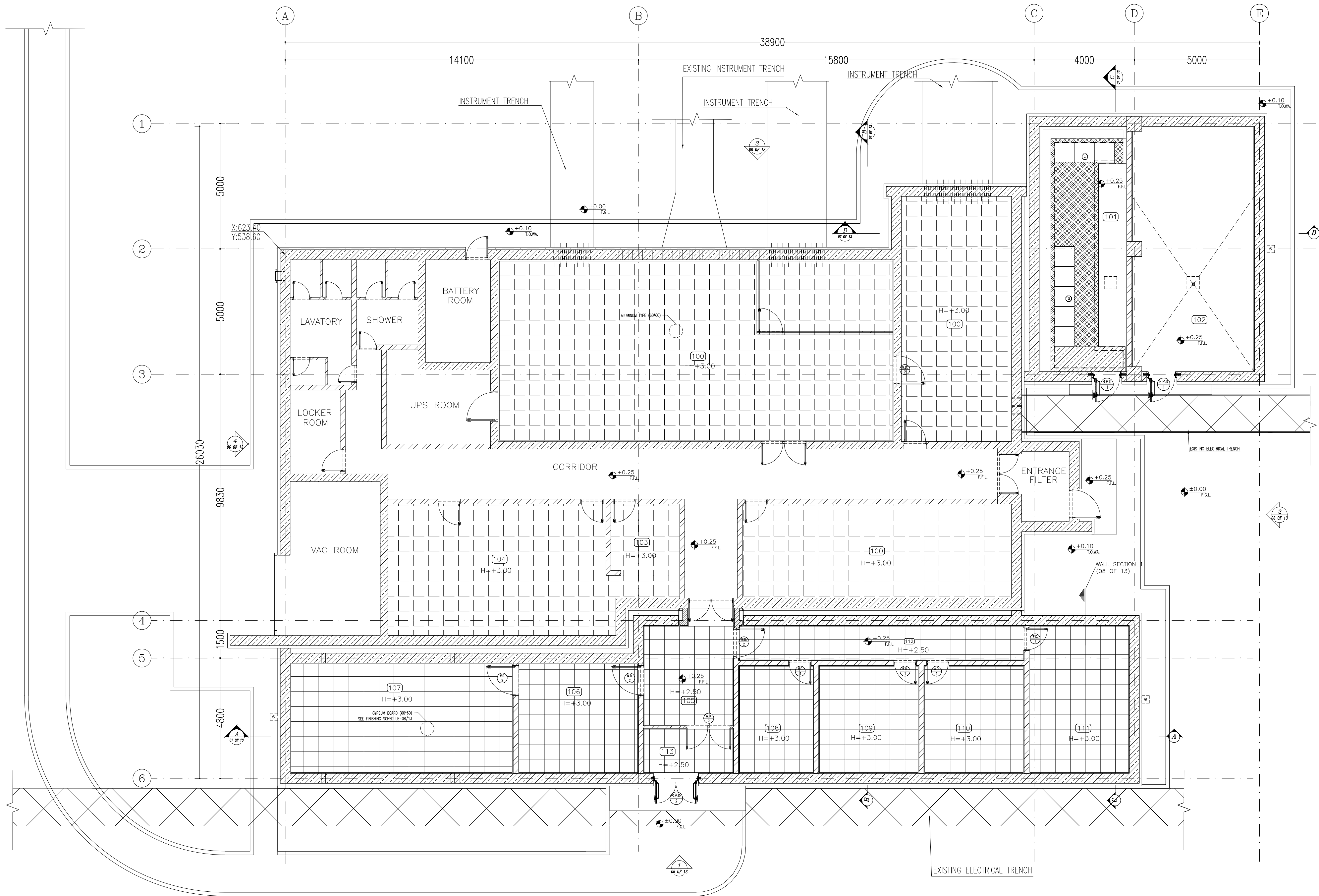
SC.1:100 4 SUSPENDED CEILING PLAN
