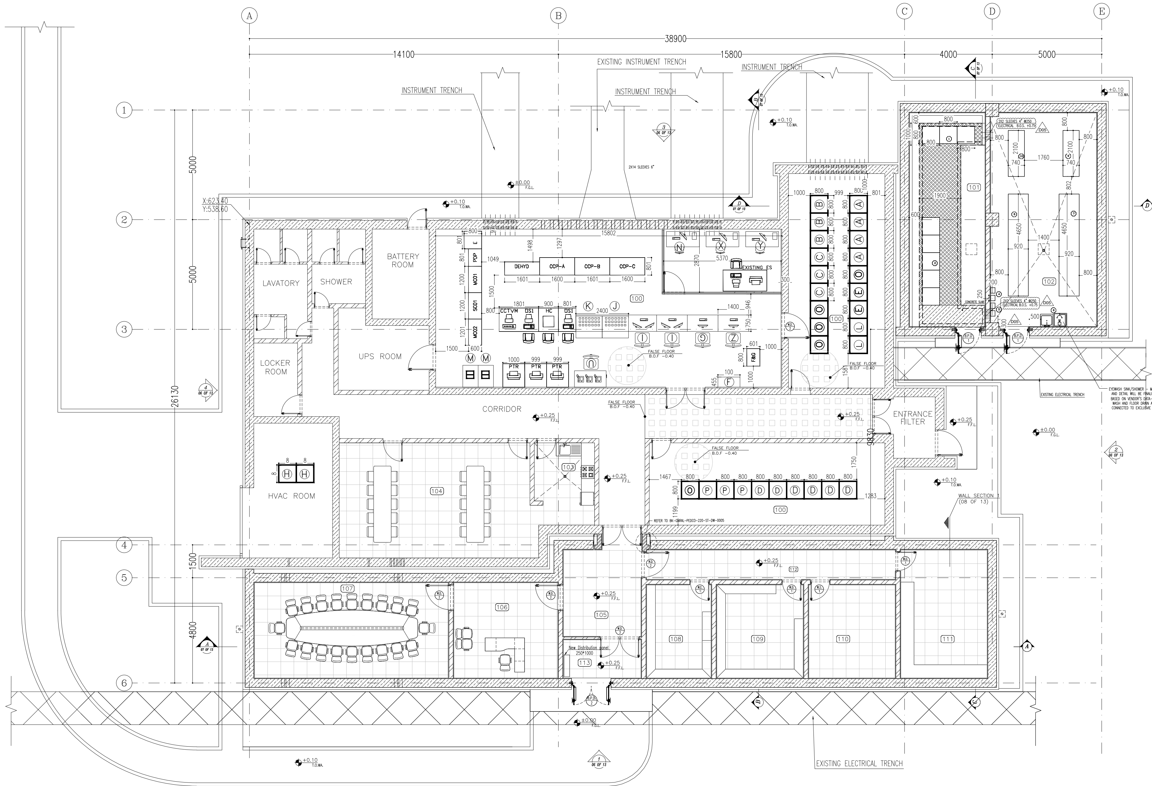
SC.1:100 3 FURNITURE & FLOORING PLAN
