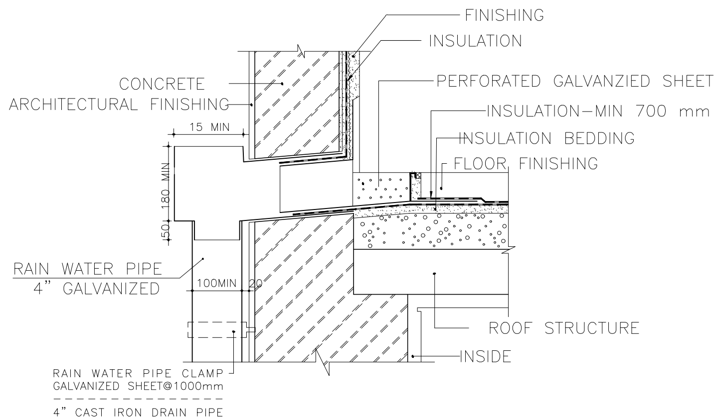
DETAIL 04 (RAIN WATER DISPOSAL DETAIL) Sc:1/10
