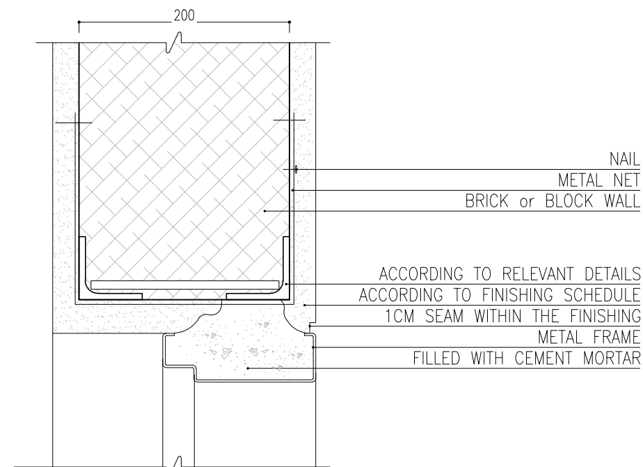
DETAIL 09 Sc:1/5
