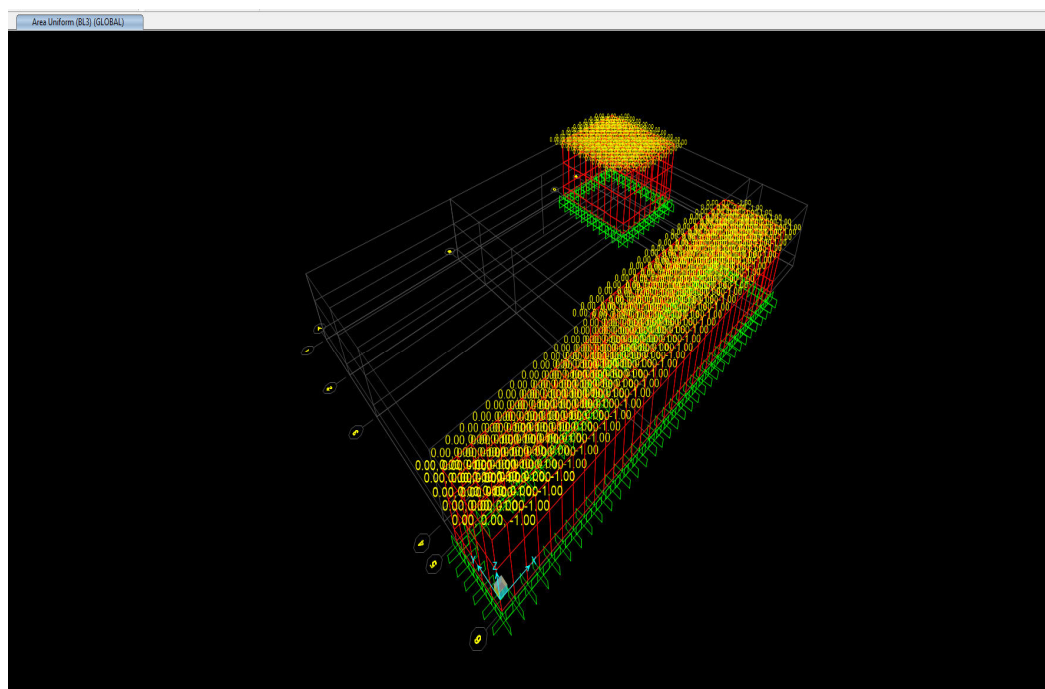
Blast Loading on Roof, BL_3 (t.m)
