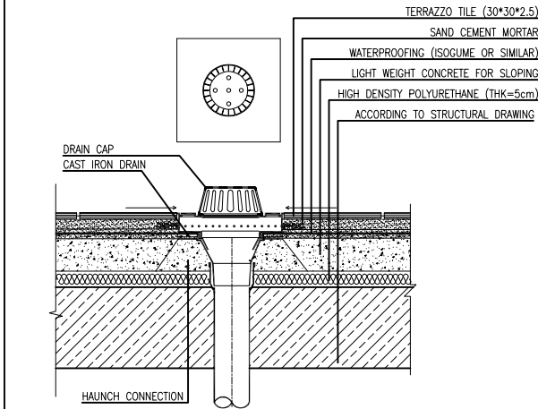
DETAIL 04 Sc:1/10
