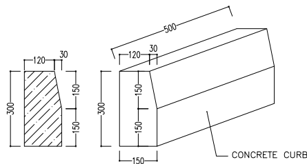
DETAIL 11 Sc:1/10
