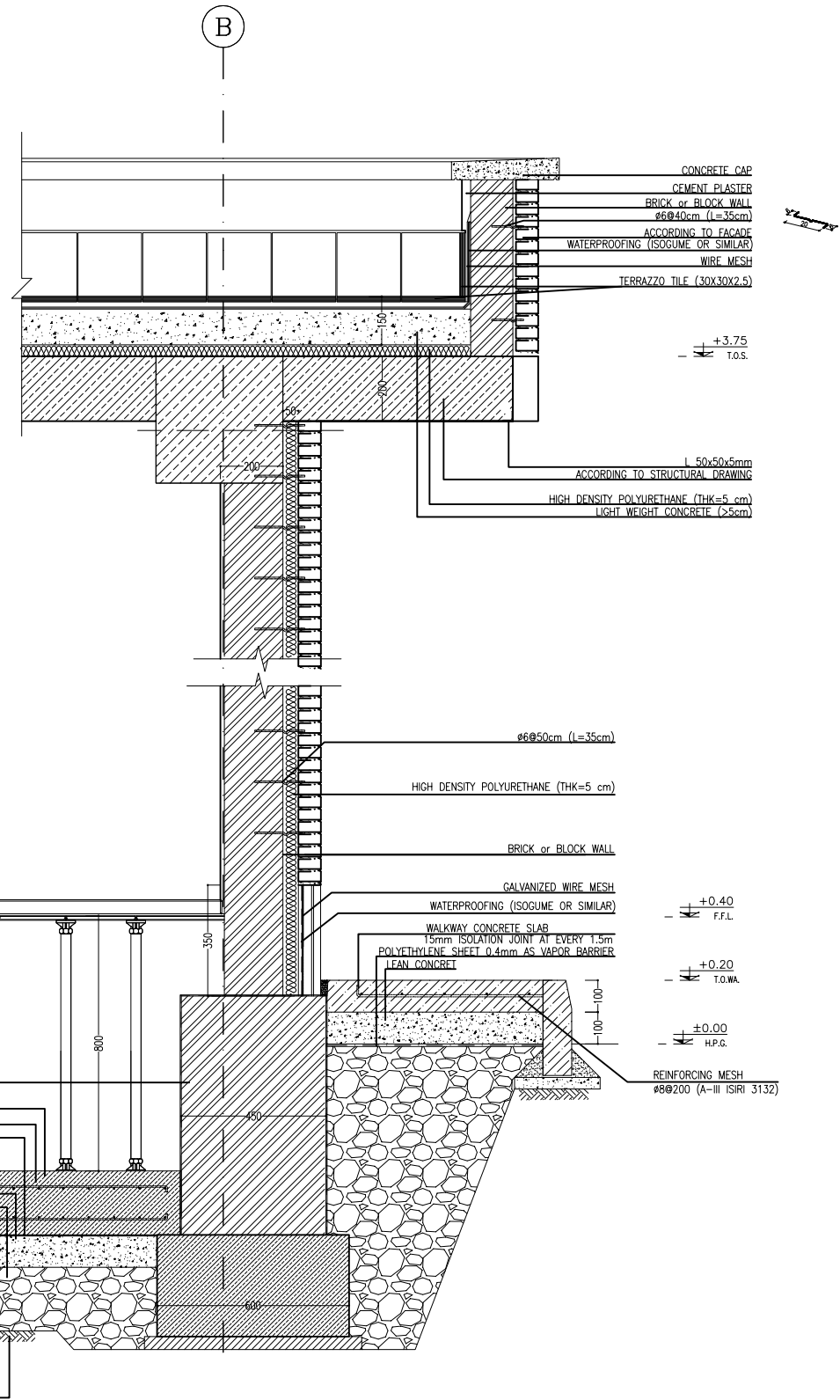
1 WALL SECTION 1 SC:1:20
