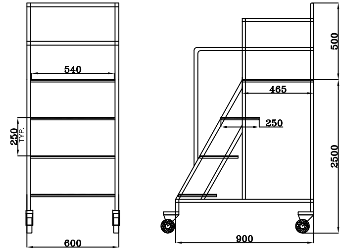
MOBILE MOTTOR ACCESS PLAT FORME
