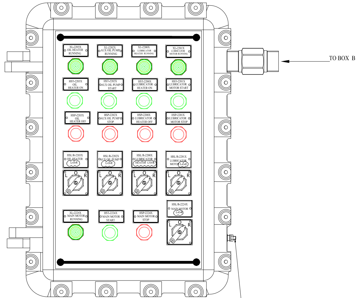
Front View
