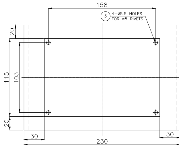
BRACKET SCALE = 1:2
