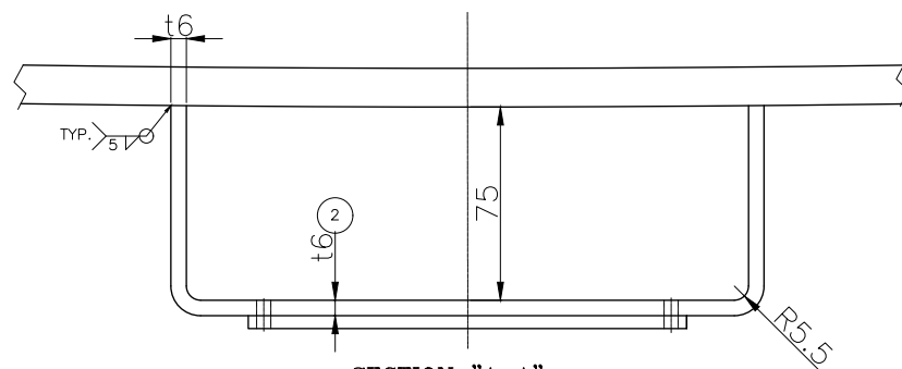
BRACKET SCALE = 1:2
