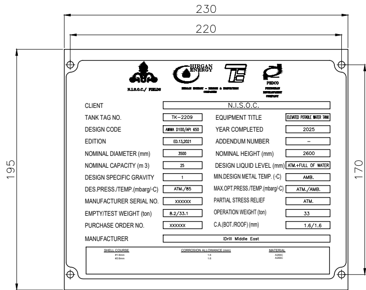
NAME PLATE SCALE = 1:1
