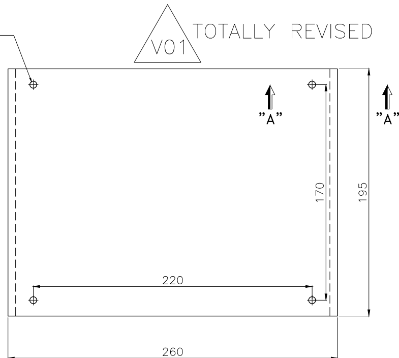
NAME PLATE HOLDER DETAIL
