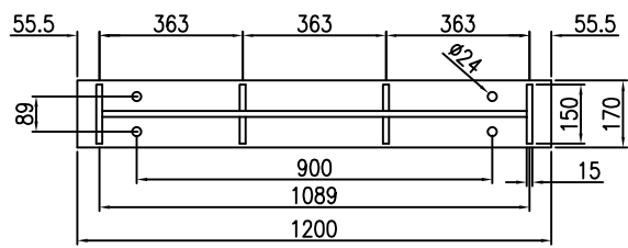
VIEW "D" FIXED SADDLE SCALE 1:20
