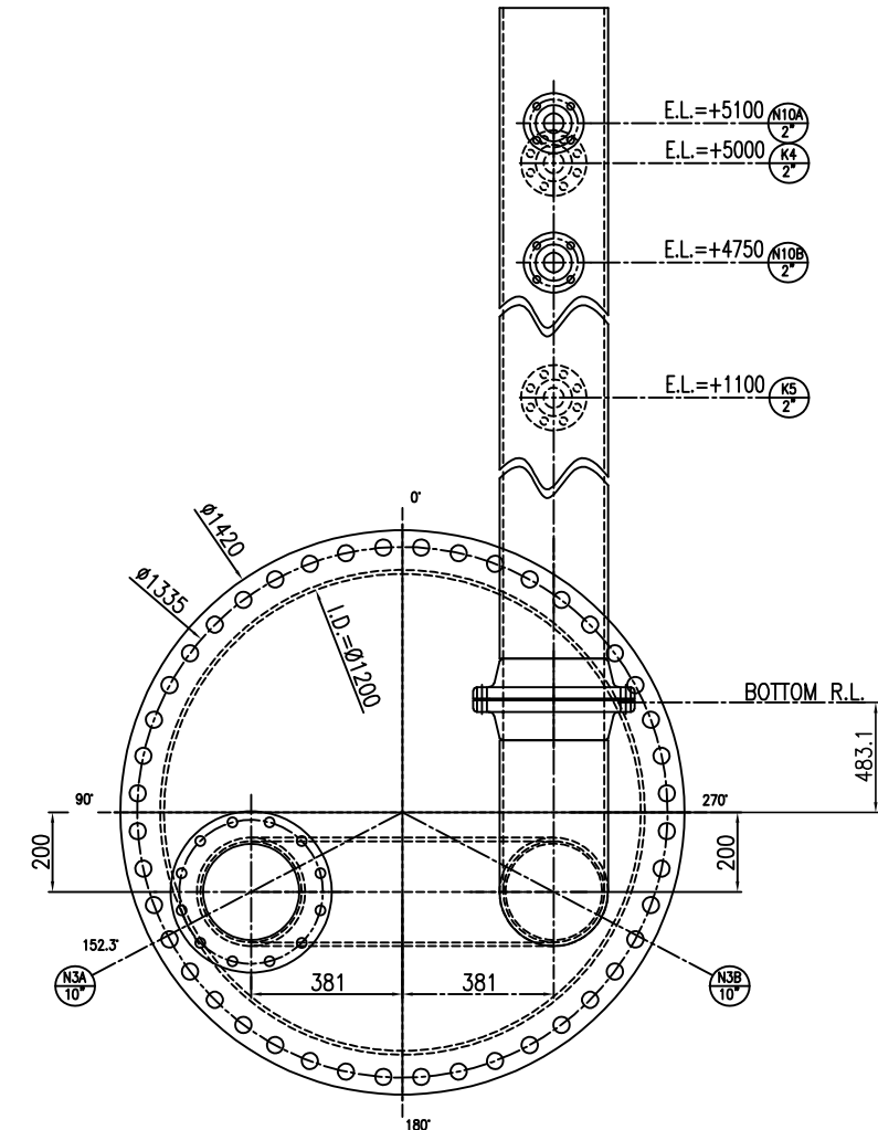
VIEW "C" SCALE 1:20
