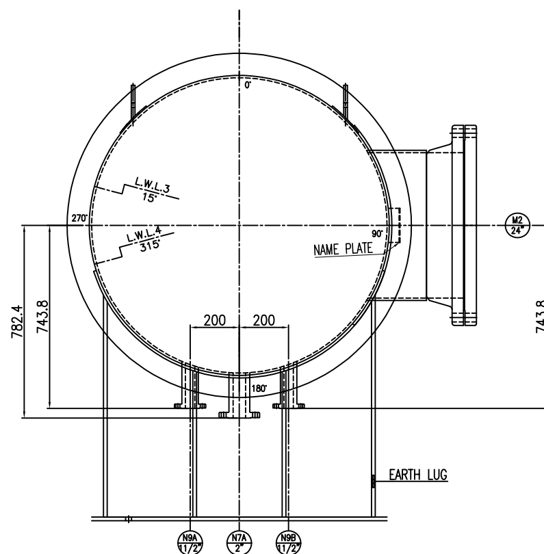
VIEW "B" SCALE 1:20
