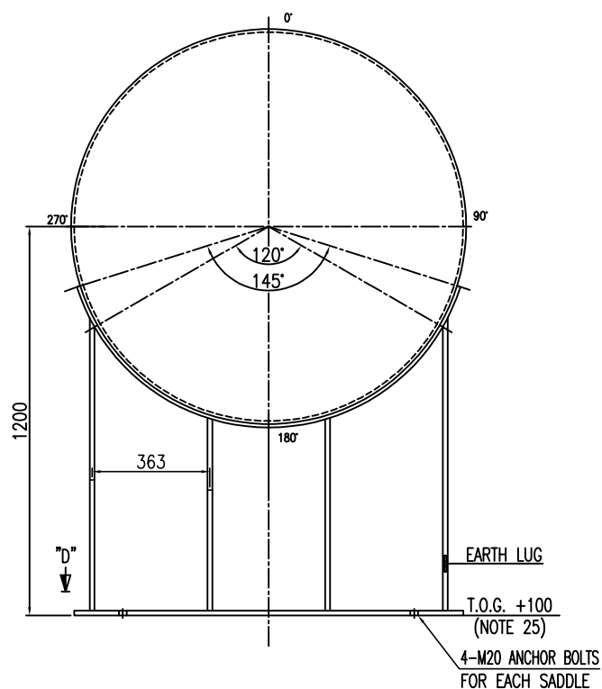
SADDLE VIEW "A" SCALE 1:20
